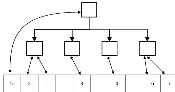
Figure 178: Redundancy in quad-tree pointers
